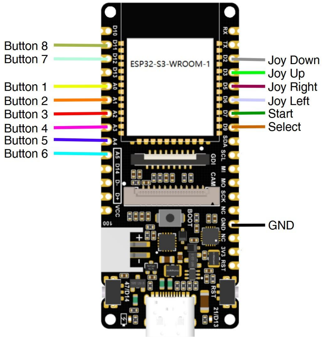
Picture 51 - ESP32-S3 DFR1145 proposed connection diagram
